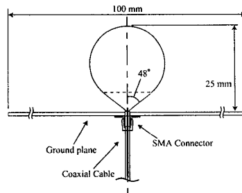
Fig. 4. Cross Section of prototype antenna.
