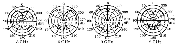
Fig. 7. Measured E-plane radiation patterns of the prototype antenna.
