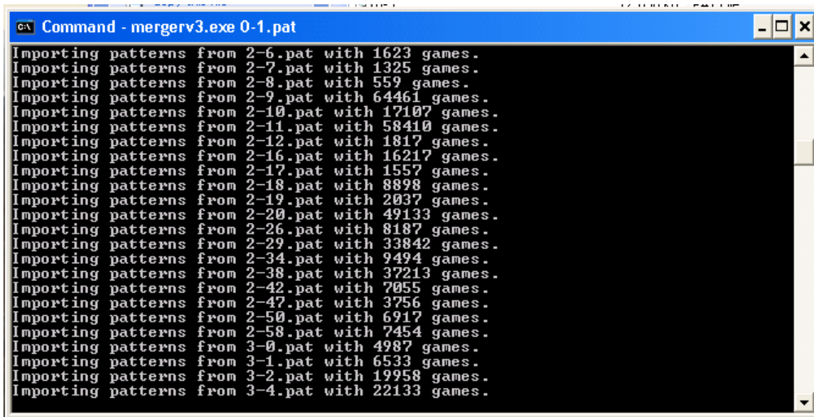
Figure 36: Mergerv3.exe running
